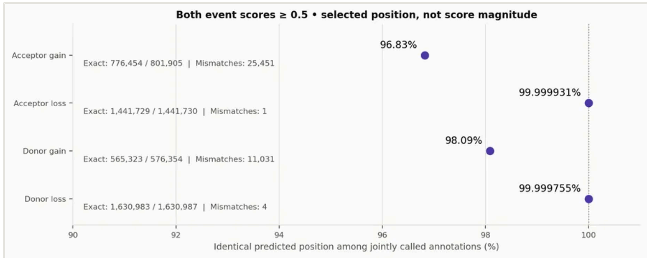
Figure 5. Jointly called gains usually select the same position. Both event scores must be \geq 0.5 . Labels give exact-position matches, eligible annotation counts and mismatches. AL has one mismatch and DL four; extra decimal places prevent rounding these results to perfect agreement. The axis spans 90–101%. Recorded masking restricts retained loss positions, but does not establish the cause of the exceptions. Calls unique to one model are excluded; shared positions do not validate splice-site use.
