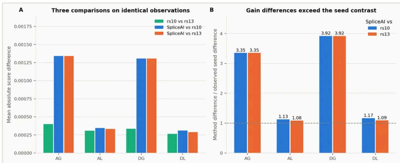
Figure 6. Gain differences exceed the observed seed contrast. A, mean absolute differences for rs10–rs13 and for each checkpoint versus SpliceAI. B, each method difference divided by the rs10–rs13 difference; one denotes equal mean differences. All contrasts use exactly the same variant–gene annotations. Two seeds provide one observed contrast, not a population estimate of training variability. Single OpenSpliceAI checkpoints and the published SpliceAI ensemble remain different comparison units.
