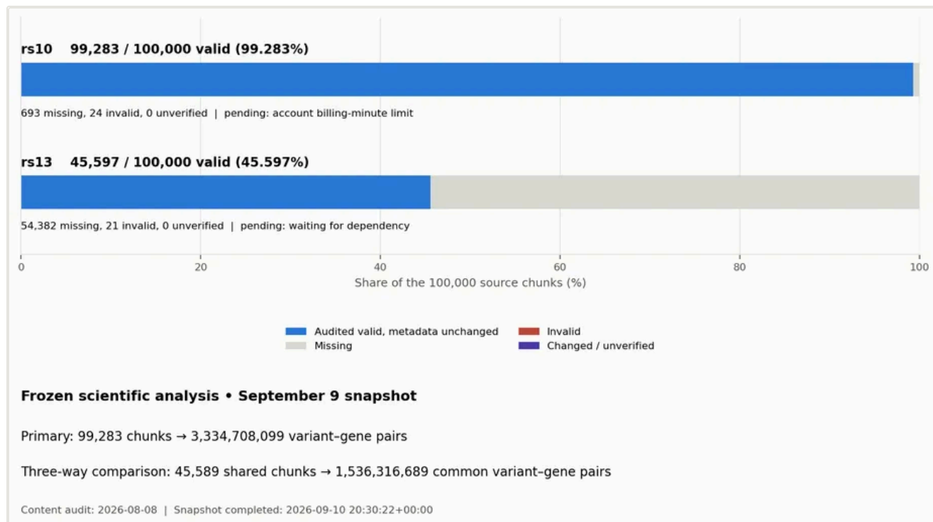
Figure 1. Inference progress and analyzed coverage. Current input/output size and modification-time checks are compared with the dated audit manifests. Unchanged metadata carries forward an audited state; it is not a new content audit. Missing, invalid and changed/unverified chunks remain separate. Job reasons are a dated scheduler observation, not a completion forecast. The lower panel shows the distinct primary and exact three-way analysis domains.
