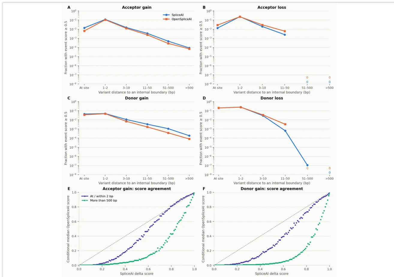
Figure 4. Annotation context distinguishes gain and loss differences. A–D, event score \geq 0.5 divided by all paired variant–gene annotations in each distance group. Counts are pooled across acceptor, donor and ambiguous boundary types before division. Both models use the same group denominator. The rate axis is logarithmic; printed zeros indicate measured zero calls. E–F, histogram-derived conditional gain-score medians at/within 2 bp versus more than 500 bp from a pooled internal boundary. The strand-aware index excludes transcript ends. Variant distance differs from selected-event distance and does not classify variants as intronic or exonic.
