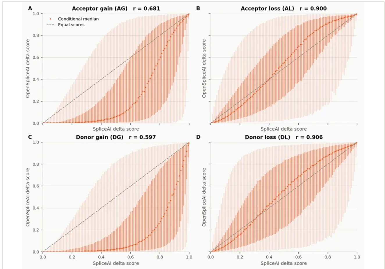
Figure 2. Loss scores agree more closely than gain scores. OpenSpliceAI scores conditional on SpliceAI scores for the primary paired variant–gene annotations. Points are medians; dark and light intervals contain the central 50% and 90%. The dashed diagonal denotes equal scores. Quantiles use stored 200-bin histograms (width 0.005); empty comparator bins remain gaps. Pearson correlations use the original scores and include shared zeros. The panels describe score agreement, not calibration against experimental outcomes.
